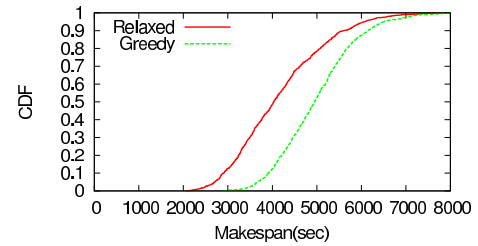
Figure 13: Comparison of the makespans of the greedy scheduler and the solution to the relaxed problem.
